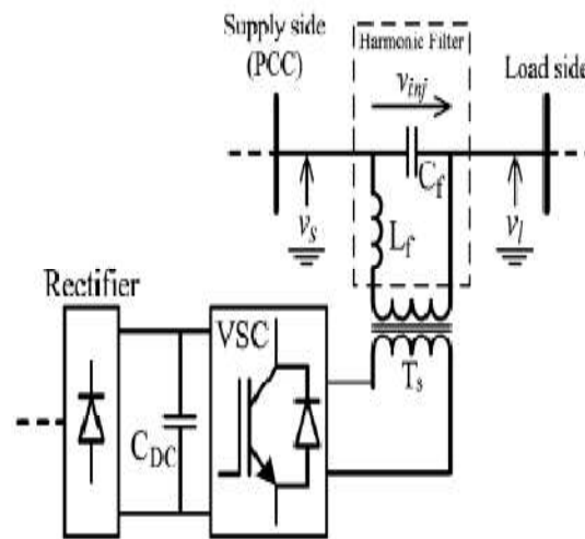
Figure.1.1.1.Schematic diagram of a DVR
