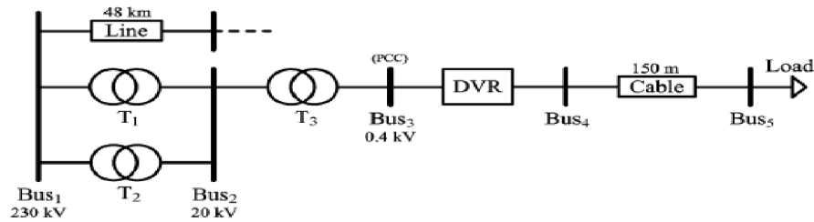
Figure 3.1. Single-line diagram of the system used for simulation studies.
