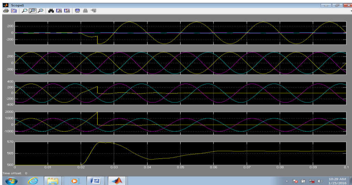
Graph.3.2.(a) Injected voltages, (b) Source voltages. (c) Load voltages. (d) Line currents. (e) DC-link voltage, during the single phase-to-ground downstream fault.
