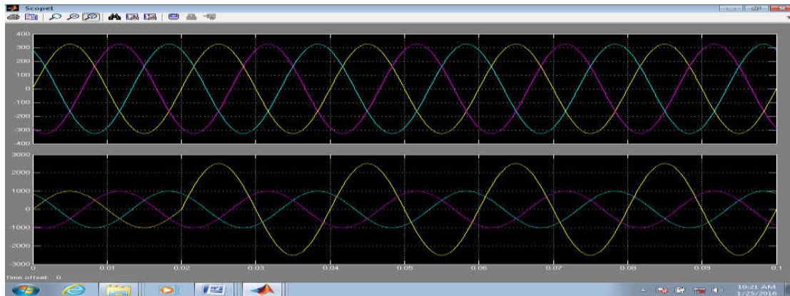
Graph.3.1 (a) Voltages at BUS 3 , (b) Fault currents, during downstream phase-to phase fault
