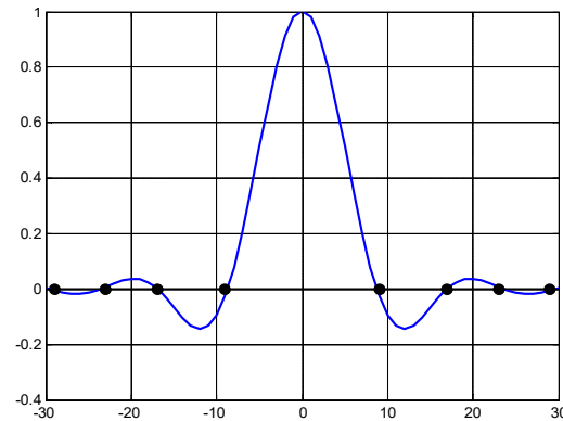
Fig.2. cancelling pulse kernel with the oversampling rate J=4. Here black dots indicates when n is taken as integer value.
