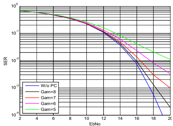
Fig.10. SER over an AWGN channel with respect to different target PAPR \gamma of 16-QAM OFDM signals in the presence of PC.
