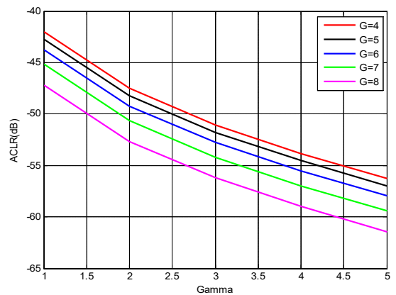
Fig.9. Graphical analysis of ACLRs with respect to multiple pulse length n under multiple target PAPR \gamma .
