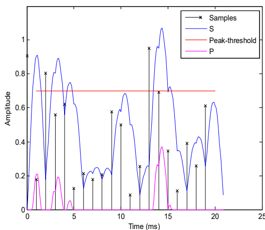
Fig.1. Waveforms associated with Peak Cancellation
