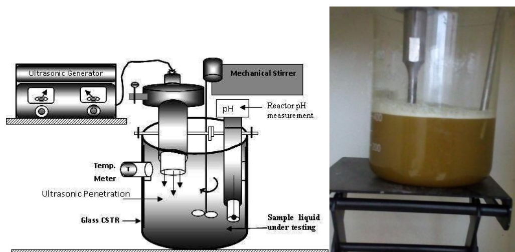
Fig : Photo of experimental setup
